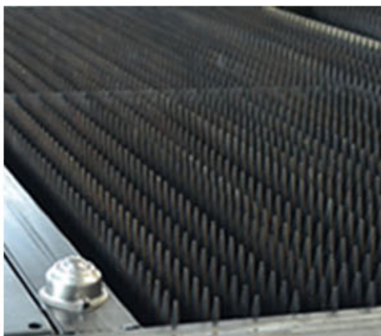
Sawtooth blade table, suitable for sheet metal cutting.
